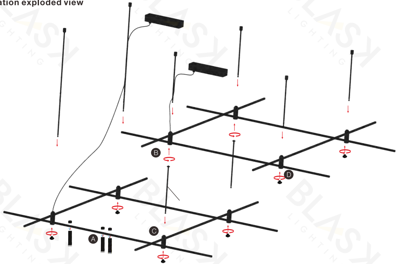
Installation exploded view
